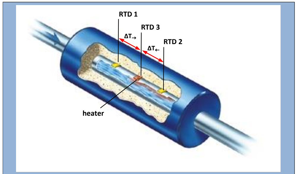
Compact inline assembly for measurement of liquid and gas flows
